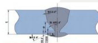
Compound Beveling According to ASME B16.[1].25
